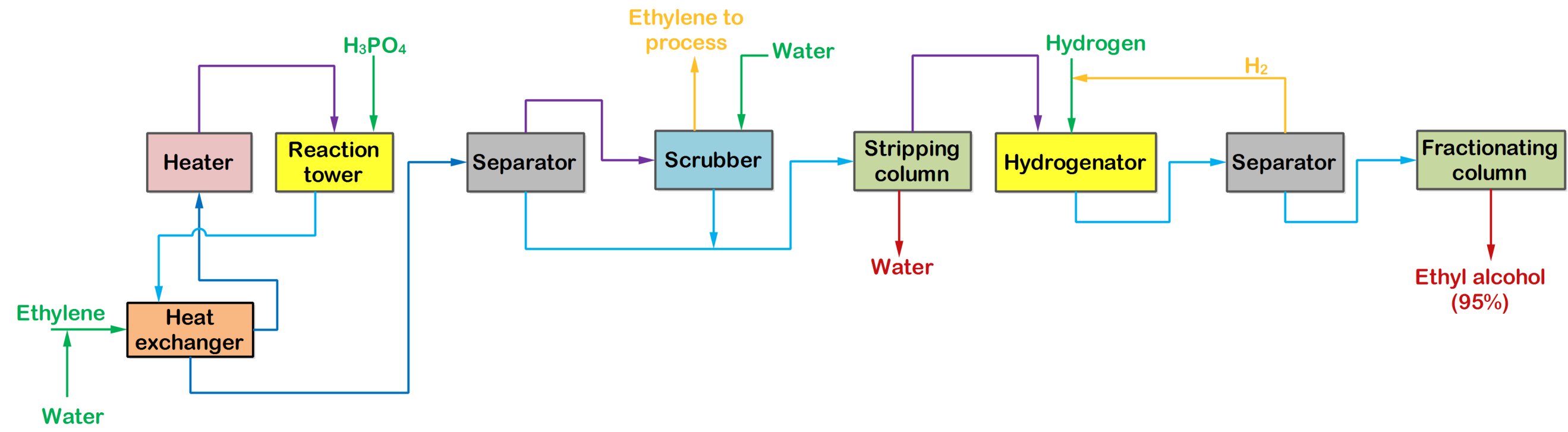
Figure: Manufacture of Industrial alcohol by catalytic hydration
